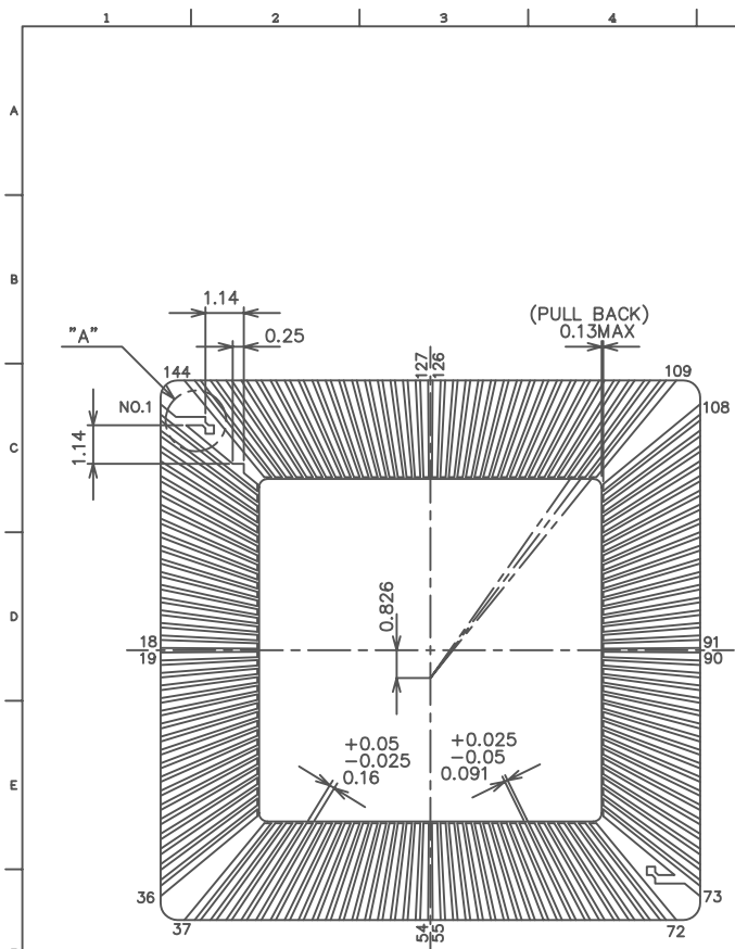
B/G PADS DETAIL
