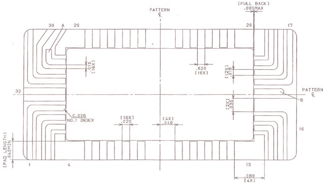
B/G PADS DETAIL
