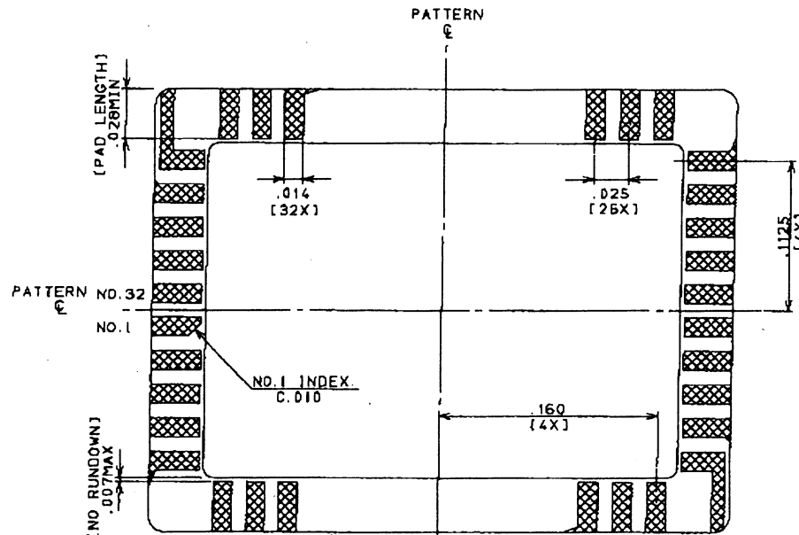
B/G PADS DETAIL
