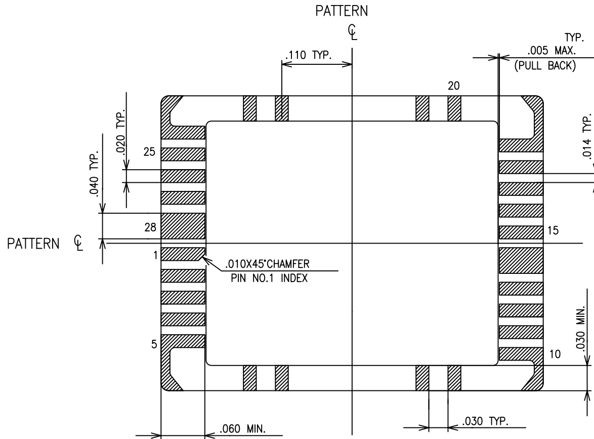
BONDING PATTERN
