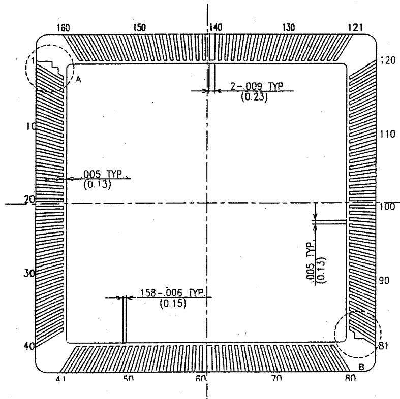
BONDING PATTERN (15:1)
