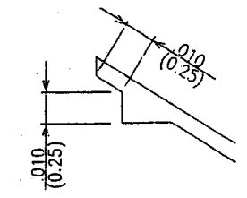
DETAIL "B" (PIN NO.81) (SCALE 45:1)
