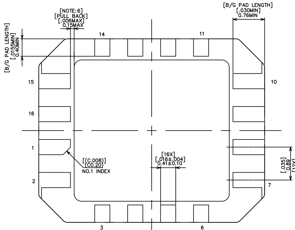
B/G PADS DETAIL
